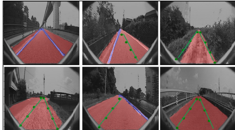
Free Space and Lane Marker Segmentation
